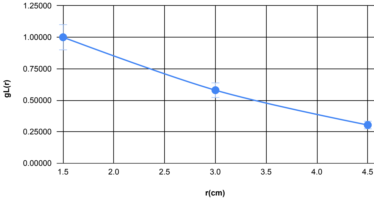
g_L(r) vs r
